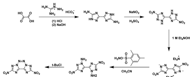
Scheme 1 Synthesis of 2,9-dinitro-bis[1,2,4]triazolo[1,5-d:5',10'-f][1,2,3,4]tetrazine, an annulated energetic system. 26,28,32
