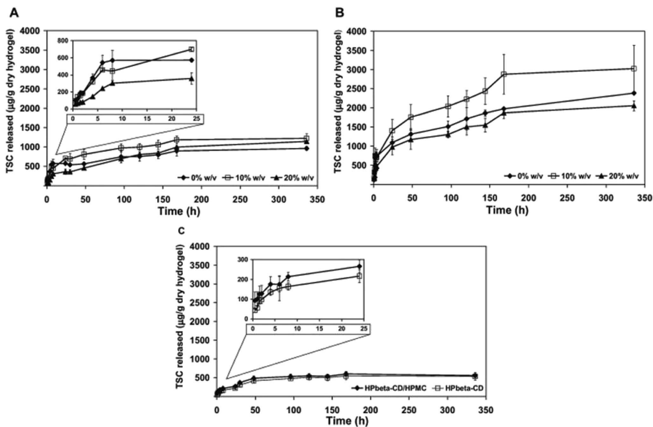
Fig. 14 Thiosemicarbazone release kinetics from different hydrogels over two weeks, at 25 °C. (A) pHEMA-co-β-CD produced by the DP method, (B) pHEMA-co-β-CD produced by the PP method and (C) HPβ-CD and HPβ-CD/HPMC SHHs. The artificial lacrimal fluid medium was replaced to maintain sink conditions every (A) 30 h, (B) 4 h and (C) 8 h. Figure insets show the release during the first 24 h. Reprinted with permission from ref. 95. Copyright (2013), Elsevier.
