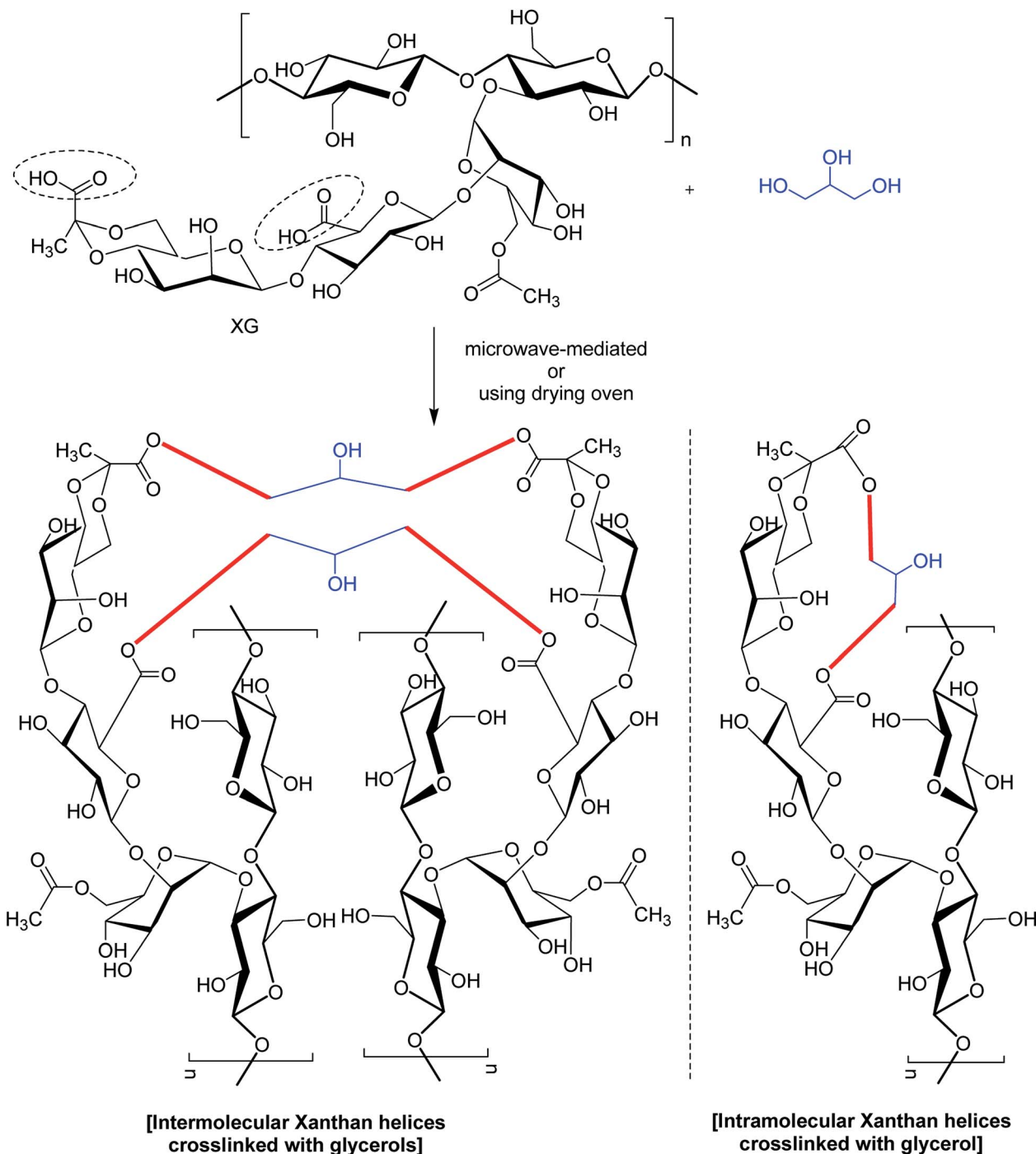
Fig. 8 Glycerol-crosslinked XG.
