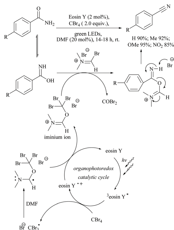
Scheme 53 Organo-photocatalytic dehydration.
