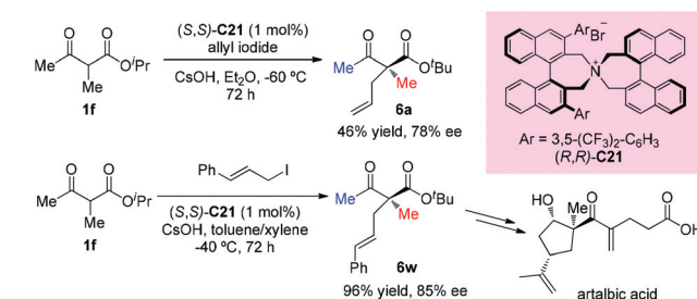
Scheme 34 Asymmetric allylation catalyzed by PTC C21.
