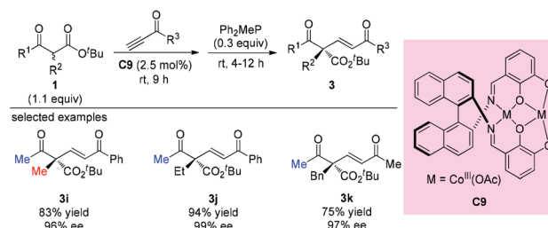
Scheme 13 Asymmetric addition of \beta -ketoesters to alkynones using a Co-Schiff base.
