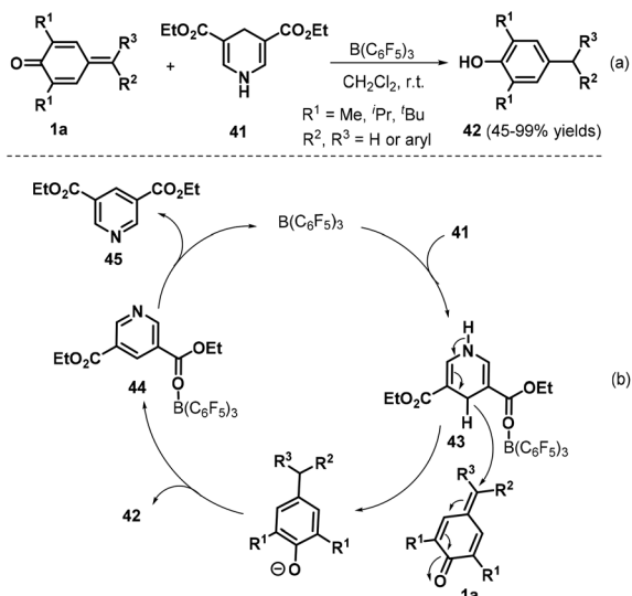
Scheme 11 \text{B(C}_6\text{F}_5)_3 -Catalyzed reduction of p -QMs.
