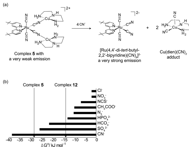
Fig. 3 (a) The detection of cyanide by complex 5 via the IDA; (b) binding strengths ( \Delta G^\circ ) of various [\text{Cu}(\text{dien})\text{--analyte}] adducts. The vertical lines represent the \Delta G^\circ values of complexes 5 and 12.
