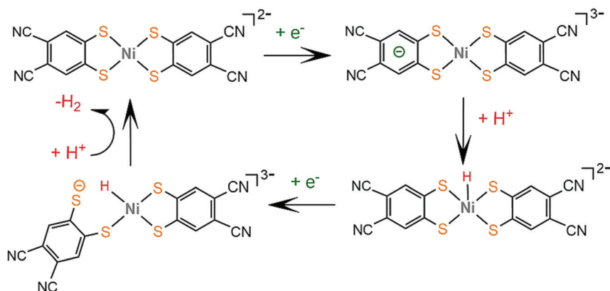
Scheme 15 Proposed ECEC mechanism catalysed by complex 24 .
