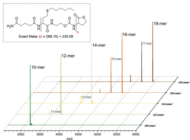
Fig. 4 MALDI-TOF spectrum of oligomer samples during the synthesis of an at -octadecamer in a single continuous run after the 10, 12, 14, 16 and 18 th reaction cycle. The peaks correspond to the sodium adduct ( [M + Na]^+ ) of the oligomers.
