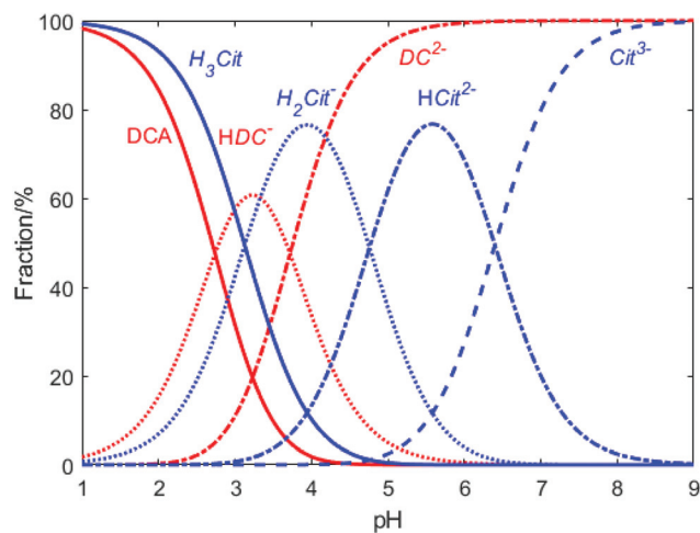
Fig. 11 Relative concentration of the different dissociation species of sodium citrate and DCA as a function of pH. H_3Cit , H_2Cit^- , HCit^{2-} and Cit^{3-} represent different forms of citrate. DCA, HDC^- and DC^{2-} represent different forms of dicarboxyacetone (according to reactions (3) and (4)). The pK_a values for citrate hydrolysis are 3.1, 4.76, 6.4, respectively; the pK_a values for dicarboxyacetone are 2.74 and 3.72 respectively.
