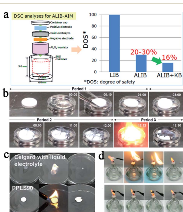
Fig. 5 (a) Schematic of the procedure of the all-inclusive microcell followed for DSC analyses and the test results of the battery with liquid and solid electrolytes, adapted with permission from ref. 62, American Chemical Society, Copyright 2017. (b) Sequential images as a function of time for contact of sintered LAGP pellet and melted Li metal at 200 °C in the glovebox, adapted with permission from ref. 71, American Chemical Society, Copyright 2017. (c) The flammability test of the Celgard separator and PPLS90 membrane, adapted with permission from ref. 75, Elsevier, Copyright 2019. (d) The flammability test of the Celgard separator, PEO, and HVTPE, adapted with permission from ref. 76, American Chemical Society, Copyright 2019.
