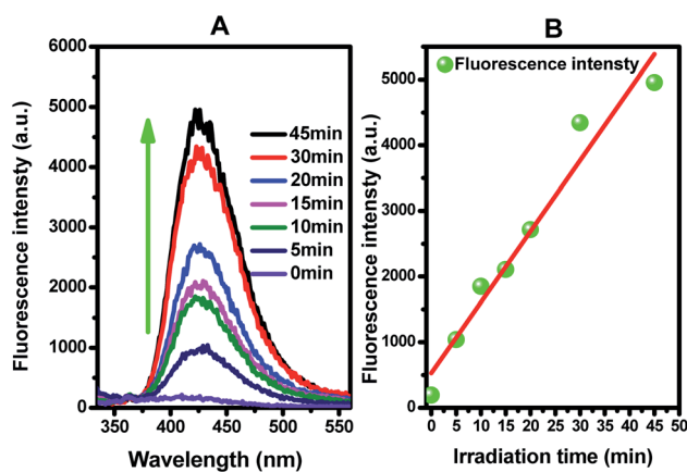
Fig. 8 (A) Fluorescence spectral changes observed during the illumination of Ti 0.7 W 0.3 O 2 /TiO 2 NCI in 0.01 M NaOH and 3 mM terephthalic acid solution (under 315 nm excitation); (B) plots showing the induced fluorescence intensities (425 nm) against light illumination time for terephthalic acid.
