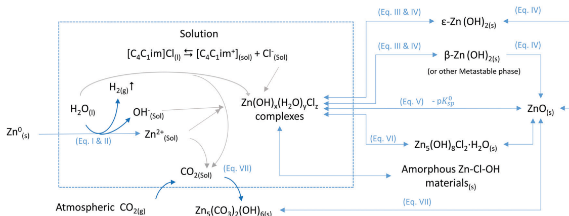
Fig. 9 General conversion paths of metallic zinc into ZnO in [\text{C}_4\text{C}_1\text{im}]\text{Cl}/\text{water} systems. Equations in the scheme are not balanced. Equations are given in the text. The predominant path and species formed will depend on the temperature and water content.
