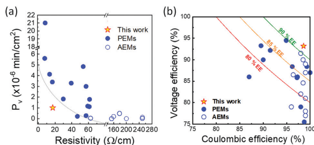
Fig. 4 (a) Trade-off between vanadium diffusivity and resistivity. (b) VRFB performance relationship among CE, VE, and EE at 40–60 \text{mA cm}^{-2} . Detailed information on the trade-off curves is available in Tables S3 and S4 (ESI † ).
