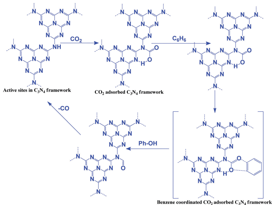
Scheme 10 Oxidation of benzene to phenol using \text{CO}_2 as an oxidant and g\text{-C}_3\text{N}_4 as a catalyst.
