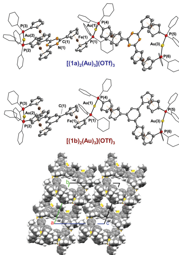
Fig. 6 Molecular structures of [(\mathbf{1a})_2(\text{Au})_3](\text{OTf})_3 (top) and [(\mathbf{1b})_2(\text{Au})_3](\text{OTf})_3 (centre). Thermal ellipsoids set at 50% probability level. For clarity, P -bound phenyl groups are depicted in wireframe style, and co-crystallised solvent, anions, and hydrogen atoms are omitted. Bottom: Space-filling model of [(\mathbf{1b})_2(\text{Au})_3](\text{OTf})_3 viewed along the crystallographic a axis; crystallographic axes of the unit cell are shown, solvent molecules are omitted.
