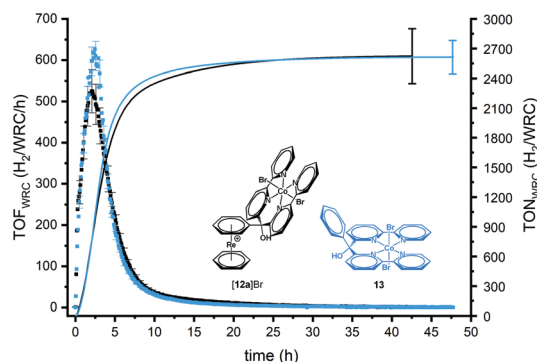
Fig. 4 Photocatalysis experiment with [\text{12a}]\text{Br} in black and the parent catalyst 13 in blue. TOF (dots) ( \text{H}_2/\text{Co}/\text{h} ) and TON (lines) ( \text{H}_2/\text{Co} ) formed as a function of time for 5 \mu\text{M} catalyst. Experimental conditions: 10 mL solution, 0.5 mM [\text{Ru}(\text{bpy})_3]\text{Cl}_2 , 0.1 M NaAsc, 0.1 M TCEP, pH 5.0, 453 nm LED irradiation.
