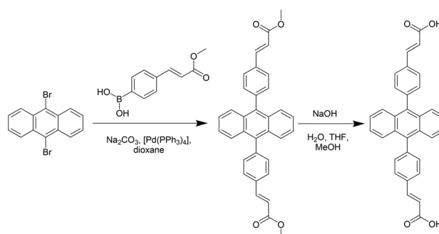
Scheme 1 Synthesis of 4,4'-(9,10-anthracenediyl)dicinamic acid (H 2 L).
