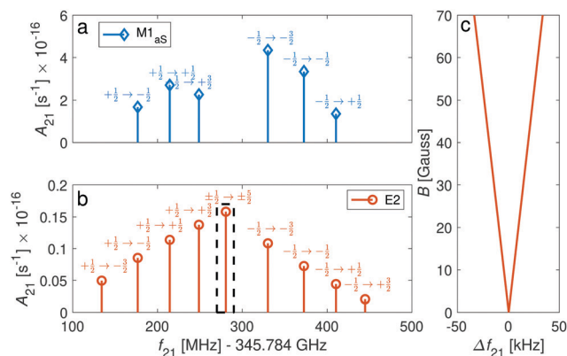
Fig. 8 Spectrum of Zeeman components of the spin-rotational transition |N = 0, J = 1/2\rangle \rightarrow |N' = 2, J' = 5/2\rangle for the l = 0 isomer. The intensities of the transitions are given in the form of Einstein A coefficients (eqn (23) and (22)) for comparison of (a) M1_{as} coupling with (b) E2 coupling. The magnetic field was assumed to be 70 G. Labels indicate the Zeeman components of the transitions. (c) Magnification of the dashed rectangle in (b) showing the stretched transitions, |J = 1/2, m = \pm 1/2\rangle \rightarrow |J' = 5/2, m' = \pm 5/2\rangle , which show a very small dependence on the magnetic field and are only separated by 66.5 kHz at 70 G. The frequency axis in (c) is referenced to the field-free line positions.
