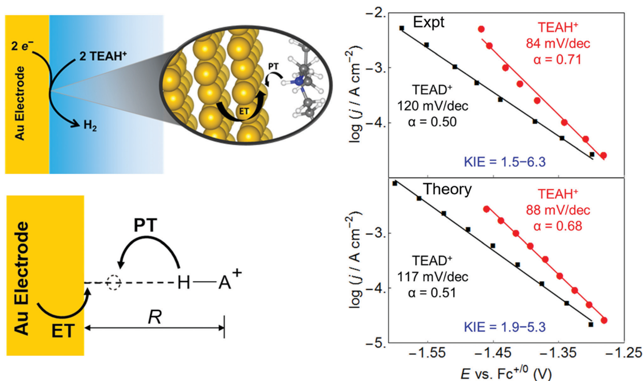
Fig. 15 Left: Schematic depiction of the PCET reaction associated with proton discharge from \text{TEAH}^+ to a gold electrode, corresponding to the Volmer reaction that is a key step in the hydrogen evolution reaction. Right: Tafel plots, which reflect the current density versus the applied potential, obtained from experimental data (upper panel) and theoretical calculations (lower panel) for the PCET reaction associated with proton discharge from \text{TEAH}^+ (red circles) or \text{TEAD}^+ (black, squares) to a gold electrode in acetonitrile. The reported Tafel slopes and electrochemical transfer coefficients, \alpha , are obtained from linear fits to the data points shown. The smallest and largest KIEs reported are the ratios between the \text{TEAH}^+ and \text{TEAD}^+ linear fits at -1.30 V and -1.46 V, respectively. Figures adapted with permission from ref. 93. Copyright 2018 American Chemical Society.
