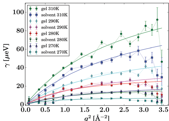
Fig. 7 Lorentzian width \gamma(q) associated with the PCM guest molecule (eqn (2), symbols). The solid lines represent fits of the jump diffusion model (eqn (3)).
