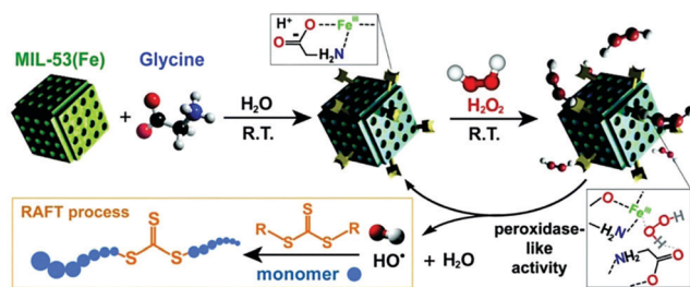
Fig. 10 Proposed mechanisms for the formation of Gly/MIL-53(Fe) and the initiation of RAFT polymerization by hydroxyl radicals. Reproduced with permission. 51 Copyright 2018 The Royal Society of Chemistry.
