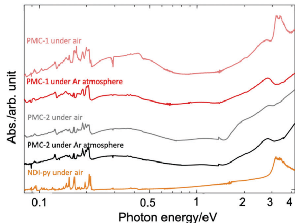
Fig. 2 Solid-state absorption spectra of PMC-2 (black line), PMC-1 (red line), and NDI-py ligand (orange line) acquired as KBr pellets.
