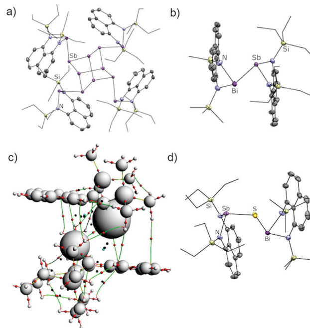
Fig. 1 (a) Single-crystal X-ray structures of (\text{EtSb})_4\text{Sb}_8 . (b) Single-crystal X-ray structures of \text{MeBiSb}^{\text{Et}} . Selected bond lengths (Å) and angles (°): Bi–Sb 2.9775(9), Bi–N 2.161(4) and 2.161(4), Sb–N 2.059(4) and 2.059(4), N–Bi–N 83.6(2), N–Sb–N 87.6(2) (c) AIM calculated bond paths and critical points for \text{MeBiSb}^{\text{Et}} . White spheres denote the nuclear basins (atoms). The vertical green lines evidence bonding interactions between the ligands in the periphery of the Bi–Sb bond. (d) Single-crystal X-ray structures of \text{MeBiSb}^{\text{Et}} . Selected bond lengths (Å) and angles (°): Sb–S 2.3838(8), Bi–S 2.5456(7), Bi–N 2.141(2) and 2.150(2), Sb–N 2.040(2) and 2.045(2), N–Bi–N 83.86(8), N–Sb–N 89.35(8). Thermal ellipsoids are shown at the 50% probability level. Hydrogens have been omitted and silyl groups are shown in wireframe for clarity.
