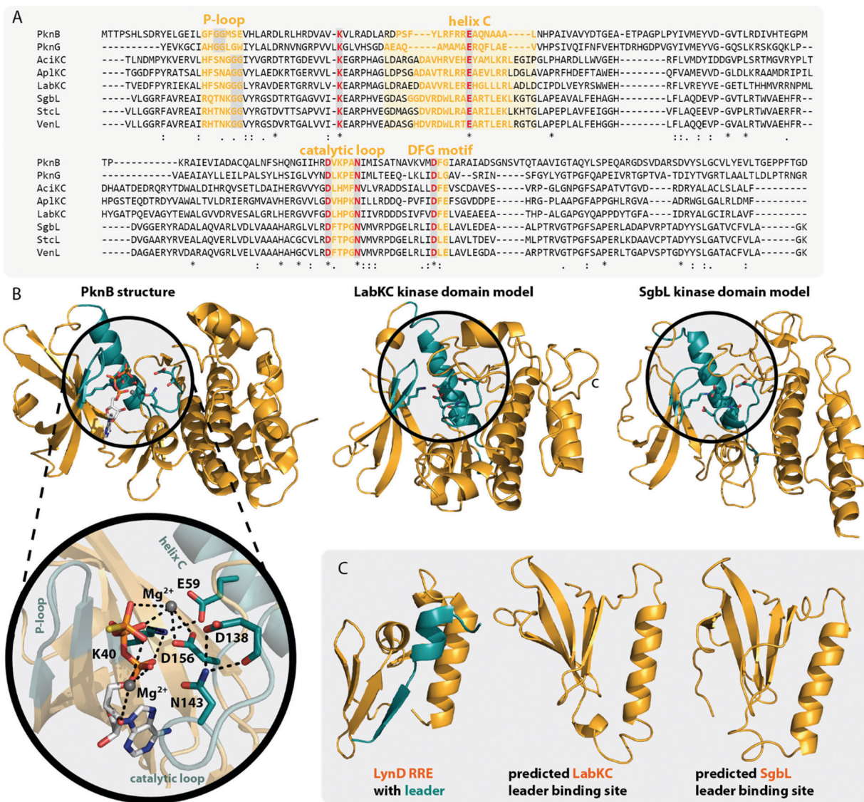
Fig. 5 (A) Excerpt of an alignment of the mycobacterial protein kinases PknB and PknG with the kinase domains of exemplary class III (AcikC, AplKC, LabKC) and class IV (SgbL, StcL, VenL) lanthipeptide synthetases. Conserved catalytic residues are shown in red and structural features important for activity are highlighted. (B) Comparison of the crystal structure of PknB binding the ATP-mimic adenosine 5'-[ \gamma -thio]triphosphate (PDB code 1MRU) with the Phyre2 models of the LabKC and SgbL kinase domains. A close up of the active site of PknB is shown. Catalytic residues and regions of importance are highlighted in teal. (C) Structure of the RRE domain of the cyanobactin heterocyclase LynD from Lyngbya aestuarii with bound leader (PDB code 4V1T) compared with the segments of the LabKC and SgbL structure models that are implied 9 in leader binding.
