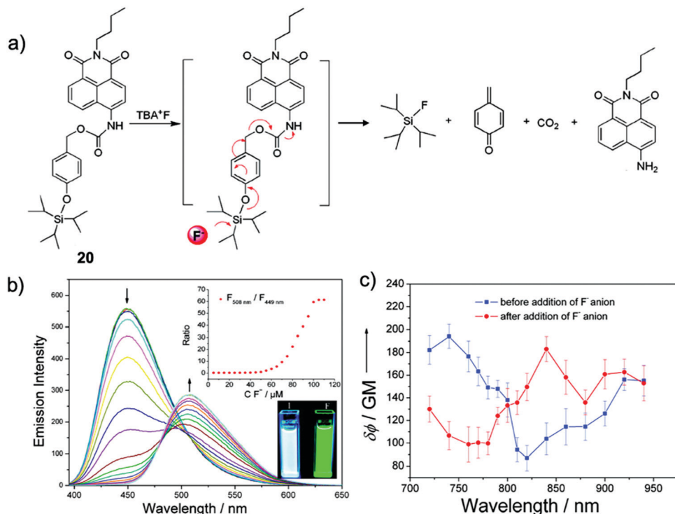
Fig. 9 Sensing mechanism and performance of 20 . (a) Reaction scheme of 20 with TBAF. (b) Fluorescence spectra of 20 (10 μM) in CH 3 CN in the presence of TBAF (0–110 μM). Insets: (upper) Ratios of fluorescent intensities at 508 and 449 nm as a function of F - concentration; (lower) fluorescence images of 20 (10 μM) before and after addition of TBAF (110 μM) in CH 3 CN. λ ex = 365 nm. (c) Two-photon action spectra of 20 (10 μM solution in CH 3 CN) before (blue line) and after (red line) addition of TBAF (110 μM). Error bars represent the standard deviation from replicate experiments ( n = 10). Reproduced with permission from ref. 39. Copyright 2011, American Chemical Society.
