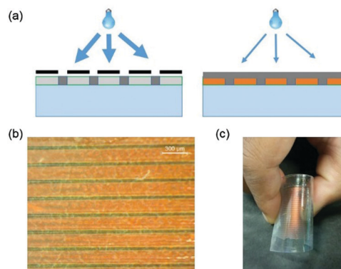
Fig. 4 (a) The production method of the anchored films. First, exposure of the LC/monomer blend was done with 405 nm light at high intensity through a mask to establish ~20 μm wide 'walls', followed by removal of the mask and exposure at 365 nm to promote vertical displacement and polymerization of the top layer. (b) Photograph of a microscopy image of the resulting polymerized film. (c) Photograph of the polymerized film on a polycarbonate substrate being bent to an extreme angle to show the adhesion and robustness of the system.
