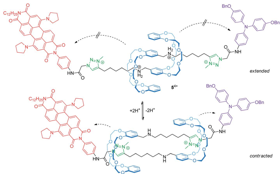
Fig. 6 Switching of the acid/base-responsive [c2]daisy chain rotaxane 5^{4+} between its extended and contracted form. Both forms show altered electrochemical properties. The dashed arrows illustrate electronic through-space interactions between the wheels and the redox-centers.
