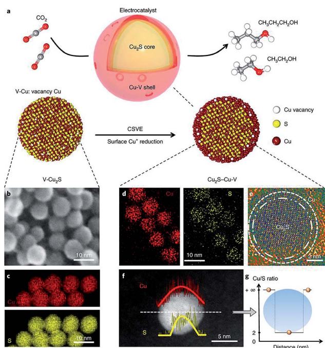
Fig. 15 (a) Schematic illustration of \text{Cu}_2\text{S-Cu-V} electrocatalyst design for \text{CO}_2 electroreduction to produce multi-carbon alcohols. (b) TEM and (c) EDS mapping of original V- \text{Cu}_2\text{S} nanoparticles; (d) EDS mapping, (e) high-resolution TEM, (f) EDS line scan and (g) the ratio of Cu/S concentration of the reduced \text{Cu}_2\text{S-Cu-V} electrocatalyst after electrochemical reduction. Reprinted from ref. 61 with permission from Nature Publishing Group.
