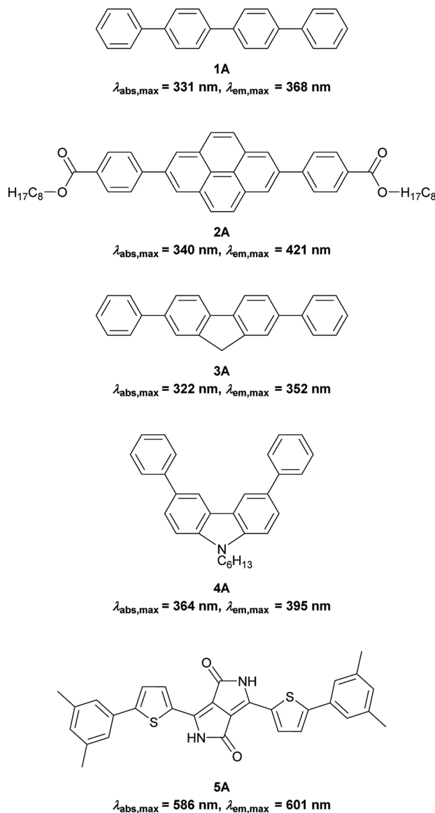
Scheme 4 Non-boron containing analogues; 1A was measured in acetone, 130 2A in toluene, 122 3A in ethyl acetate, 132 4A in MeCN 131 and 5A in DMSO.
