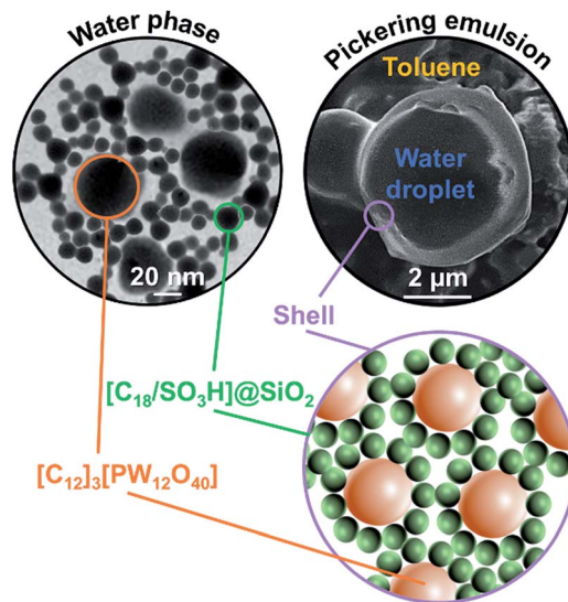
Fig. 4 TEM micrograph of [C 12 ] 3 [PW 12 O 40 ] and [C 18 /SO 3 H]@SiO 2 NP mixture (3.6 wt%, \phi = 0.5) after dispersion in water (left) and cryo-SEM micrograph of water/toluene emulsions (1/1 v/v) of [C 18 /SO 3 H]@SiO 2 /[C 12 ] 3 [PW 12 O 40 ] mixtures (3.6 wt%, \phi = 0.5, 11 500 rpm, right). The inset shows a representation of the NPs in water and at the surface droplets.
