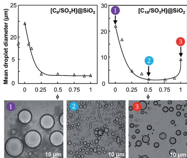
Fig. 3 Evolution of the droplet size (S.D. = 10%) as a function of the [C n /SO 3 H]@SiO 2 mass fraction ( \phi ) for water/toluene Pickering emulsions (1/1 v/v) stabilized by [C n /SO 3 H]@SiO 2 and [C 12 ] 3 [PW 12 O 40 ] NPs (3.6 wt%, 11 500 rpm). The insets present the micrographs of the W/O emulsions.
