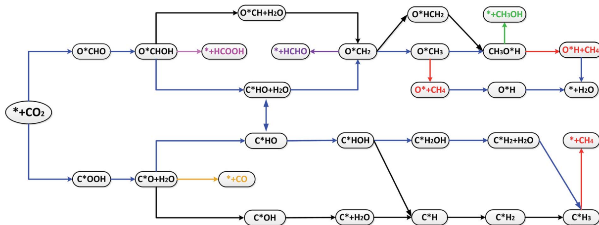
Scheme 1 Most likely reaction pathways for the electroreduction of CO 2 on TM-B p12 .
