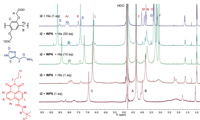
Fig. 8 ^1\text{H} -NMR spectra (500 MHz, \text{D}_2\text{O} , 0.5 mM) of the indicator displacement of i2-WP6 mixture in the presence of histamine in different concentrations. The uppermost spectrum is a mixture of i2 and histamine.
