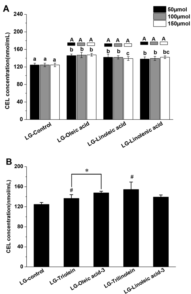
Fig. 2 Effects of fatty acids (FAs) and triglycerides (TGs) on the CEL formation in model systems. (A) The effects of different unsaturation degree and concentration of FAs on the CEL formation; (B) the effects of different TGs on the CEL formation; different lowercase letters indicate significant differences ( p < 0.05 ) among different unsaturation degree of FA (same addition level), while different capital letters indicate significant differences ( p < 0.05 ) among different addition levels (same FA). (*) p < 0.05 , significantly different between compared samples. (#) p < 0.05 , significantly different from LG-control. LG-triolein, model system added with triolein; LG-trilinolein, model systems added with trilinolein. LG-oleic acid-3, model system added with 150 μmol oleic acid; LG-linoleic acid-3, model system added with 150 μmol linoleic acid.
