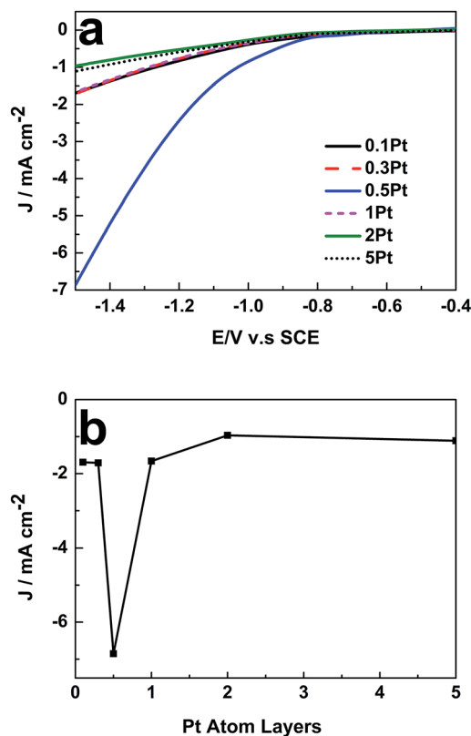
Fig. 3 Influence of \theta_{\text{Pt}} on the LSV curves of (a) 49 nm Au@Pd@Pt NRs measured in 0.1 M KHCO 3 (pH = 6.8). Scan rate: 50 mV s -1 ; current density of (b) 49 nm Au@Pd@Pt NRs at -1.5 \text{ V vs. SCE} with different \theta_{\text{Pt}} .
