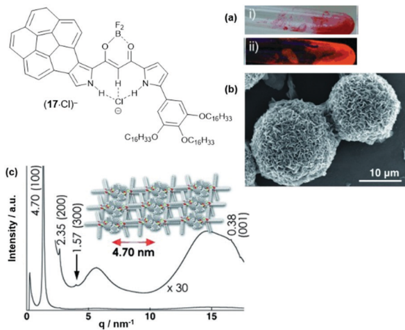
Fig. 17 Schematic representation of the \pi -electronic anion ( 17\text{-Cl}^- ). (a) Photographs of ( 14\text{a})(17\text{-Cl} ) in 1,4-dioxane under visible (i) and UV light (ii). (b) SEM image of the precipitated ( 14\text{a})(17\text{-Cl} ). (c) XRD pattern of ( 14\text{a})(17\text{-Cl} ) at 80\text{ }^\circ\text{C} on cooling from the Iso phase; the proposed supramolecular structure of the assembly is also shown. 55 Figure reproduced with kind permission; © 2013 Wiley-VCH.
