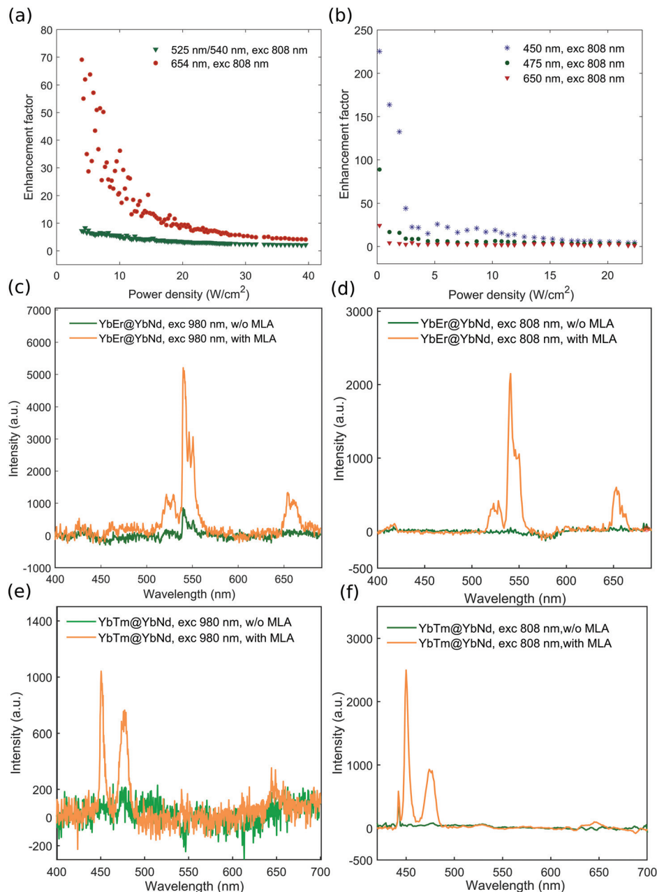
Fig. 3 Excitation intensity dependent enhancement factors induced by the addition of MLA of different emission bands of (a) \text{NaYF}_4:20\%\text{Yb}^{3+},2\%\text{Er}^{3+}@20\%\text{Yb}^{3+},30\%\text{Nd}^{3+} and (b) \text{NaYF}_4:20\%\text{Yb}^{3+},0.5\%\text{Tm}^{3+}@20\%\text{Yb}^{3+},30\%\text{Nd}^{3+} nanoparticles under 808 nm CW excitation. UCL spectra of \text{NaYF}_4:20\%\text{Yb}^{3+},2\%\text{Er}^{3+}@20\%\text{Yb}^{3+},30\%\text{Nd}^{3+} nanoparticles under (c) 980 nm and (d) 808 nm CW excitation with and without MLA light modulation (average excitation intensity: 0.1 \text{ W cm}^{-2} ). UCL spectra of \text{NaYF}_4:20\%\text{Yb}^{3+},0.5\%\text{Tm}^{3+}@20\%\text{Yb}^{3+},30\%\text{Nd}^{3+} nanoparticles under (e) 980 nm and (f) 808 nm CW excitation with and without MLA light modulation (average excitation intensity: 0.1 \text{ W cm}^{-2} ).
