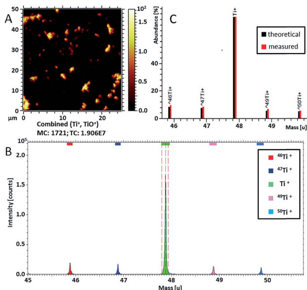
Fig. 4 Results of ToF-SIMS analysis of TiO 2 NPs in delayed extraction mode. (A) Lateral yield distribution overlay of representative Ti-containing secondary ion species. (B) Measured isotopic distribution of Ti + , all isotopes of titanium are clearly visible in the spectra and are in agreement with the natural abundance pattern as shown in (C).
