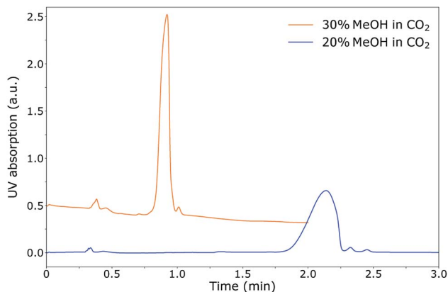
Fig. 3 UV chromatogram of the SFC separation of ManNac in water (0.78 M, 0.5 \mu L injection volume) on a 2-PIC column (Waters) at 60 ^{\circ} C, 120 bar and a flow rate of 1.5 ml min ^{-1} . The top graph was separated with a mobile phase of 30% MeOH in CO 2 , and the bottom graph with 20% MeOH in CO 2 . The sharpest peak is obtained with 30% MeOH in CO 2 .
