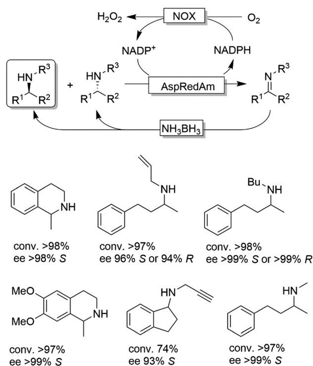
Scheme 11 CD-OS of amines exploiting the reversibility of reductive aminases. In situ \text{NADP}^+ regeneration was accomplished using \text{NADPH} oxidase (NOX). AspRedAm: reductive aminase from Aspergillus oryzae .
