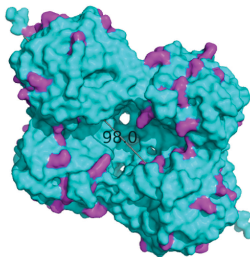
Fig. 4 MeHNL tetramer surface representation (longest extension: 98.0 Å). 60 Surface lysine residues are highlighted in magenta. X-ray structure 1DWP36 was obtained from the PDB 38 and the image was created using the PyMOL Molecular Graphics System. 37
