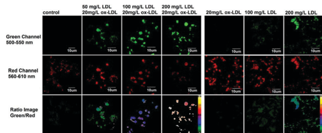
Fig. 84 Fluorescence images of stained (probe 54 , 1 \mu M for 5 min) macrophage cells being incubated with ox-LDL (20 mg L -1 ) and different amount of LDL (50–200 mg L -1 ) for 24 h, cells are stained with probe 54 at the 12th hour. Copyright 2015 American Chemical Society.
