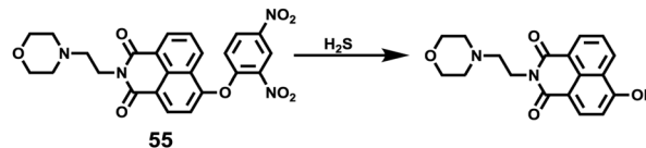
Scheme 42 Fluorescent probe 55 for H 2 S.
