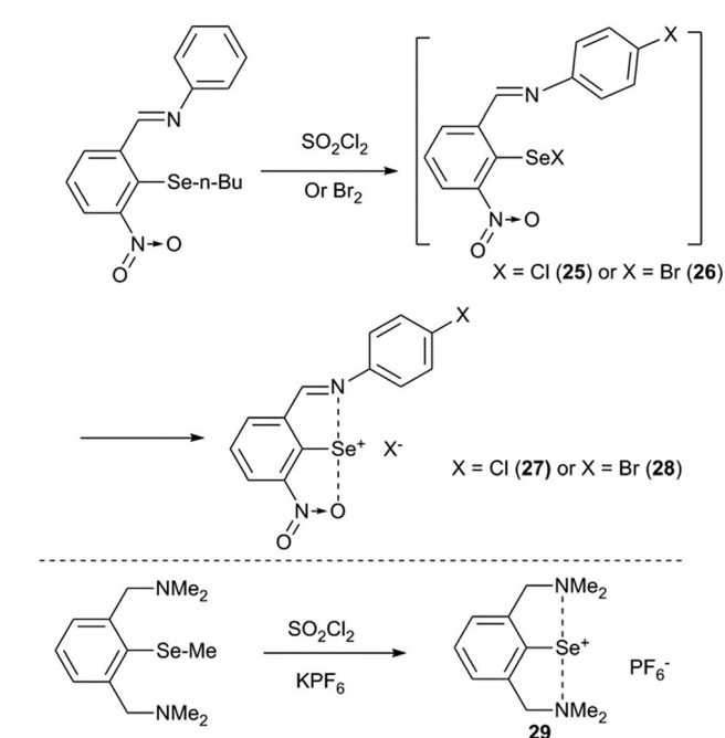
Fig. 9 Ionization of selenenyl halides.
