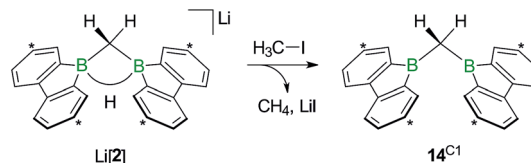
Scheme 11 The addition of H 3 C-I to Li[2] furnishes the bis(9-borafluorenyl)methane 14 C1 . Carbon atoms marked with asterisks bear t Bu substituents.
