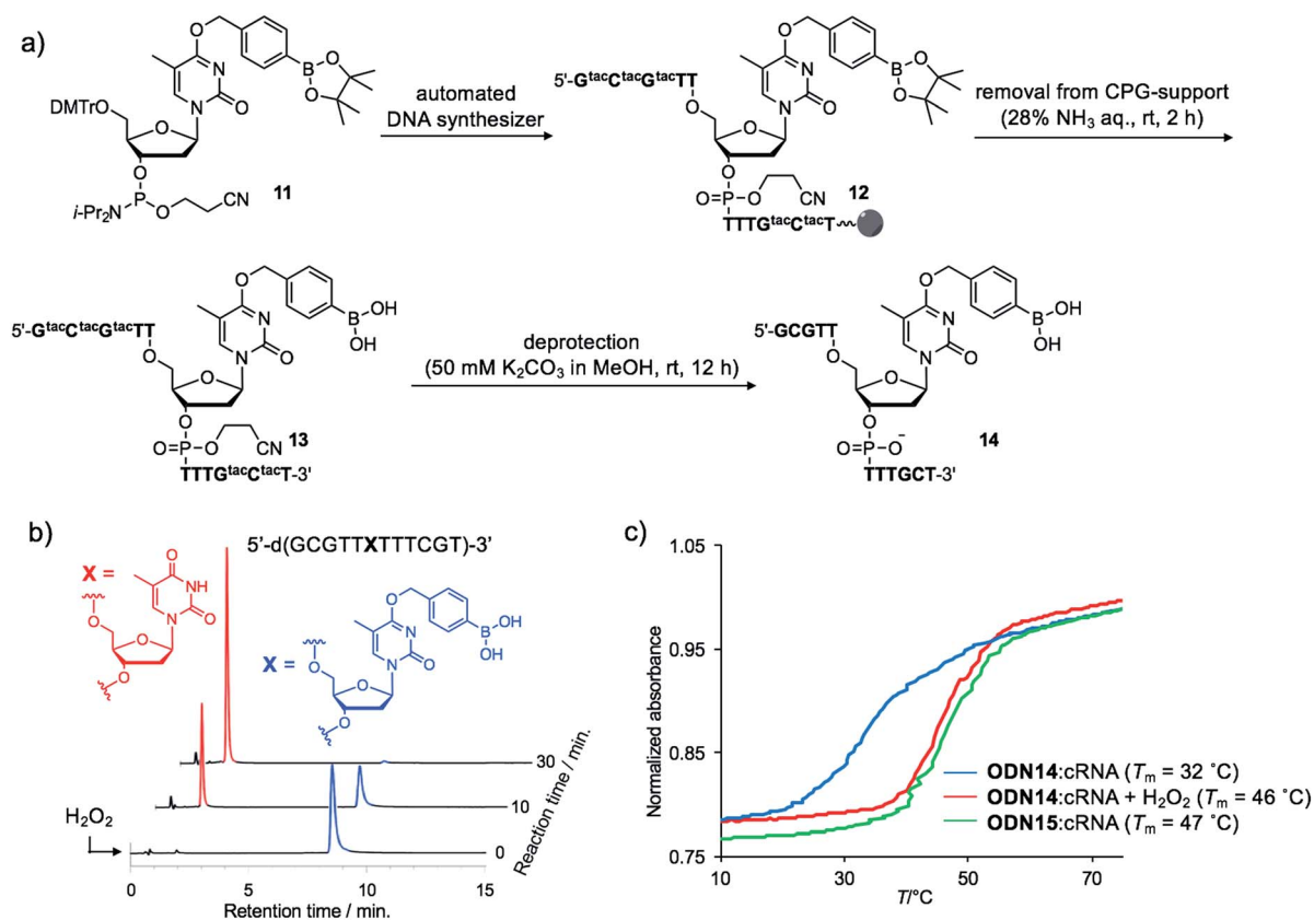
Fig. 3 (a) Synthetic scheme of boronated ODN. tac = tert-butylphenoxycetyl. (b) HPLC chromatograms of ODN14 after H 2 O 2 addition at different time points. (c) Thermal melting curves of the duplex formed between ODN14 and complementary RNA in the presence or absence of H 2 O 2 .
