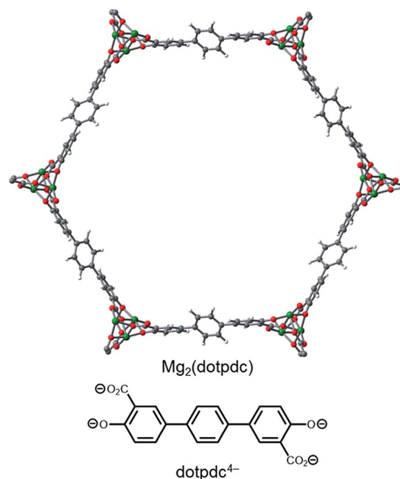
Fig. 7 Structure of the organic linker \text{dotpdc}^{4-} = 4,4''\text{-oxido-[1,1':4',1''-terphenyl]-3,3''-dicarboxylate} and a model of the hexagonal pore of Mg_2(\text{dotpdc}) . Green, grey, red, and white spheres correspond to Mg, C, O, and H, respectively.
