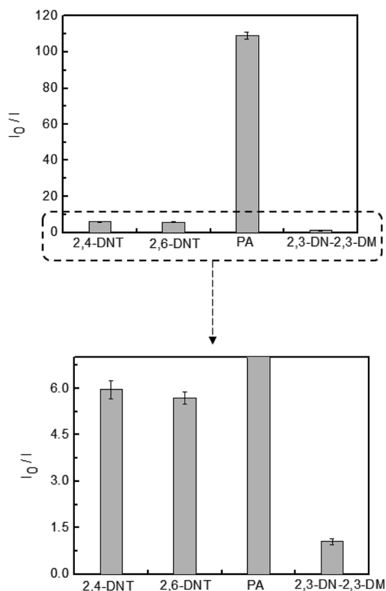
Fig. 5 Relative changes in fluorescence intensity of TPE-CMP ( 0.375 \text{ mg mL}^{-1} in \text{CH}_2\text{Cl}_2 ) upon exposure to 2,4-DNT, 2,6-DNT, PA, and 2,3-DN-2,3-DM. [\text{Explosives}] = 2.5 \times 10^{-3} \text{ M} . Excitation wavelength 330 nm. I_0 and I represent fluorescence intensity at 550 nm before and after exposure to explosives, respectively.
