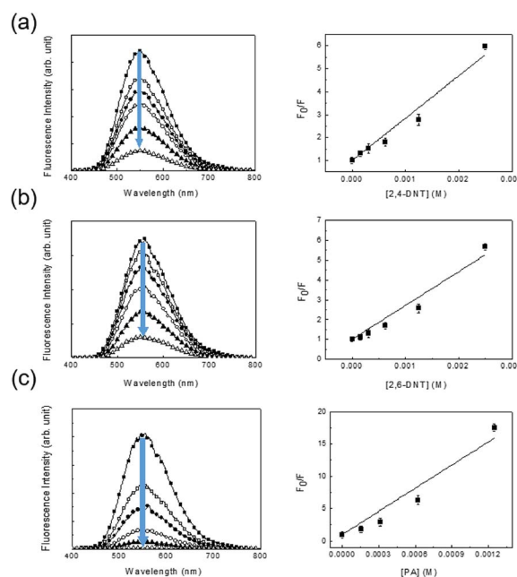
Fig. 6 Changes in the fluorescence of TPE-CMP ( 0.375 \text{ mg mL}^{-1} in \text{CH}_2\text{Cl}_2 ) with various concentrations of 2,4-DNT (a); 2,6-DNT (b); PA (c). Exposure time 5 min. [\text{Explosives}] = 0 ; 1.56 \times 10^{-4} ; 3.13 \times 10^{-4} ; 6.25 \times 10^{-4} ; 1.25 \times 10^{-3} ; 2.5 \times 10^{-3} \text{ M} . Excitation wavelength 330 nm. Right figures: Stern–Volmer plots of the fluorimetric titration. F_0 and F represent fluorescent intensity at 550 nm before and after exposure to explosives, respectively.
