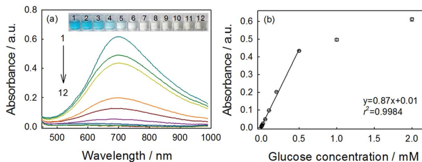
Fig. 5 UV-vis spectra (a) of different concentrations of glucose in the presence of 0.05 mg \text{mL}^{-1} GOx, 0.75 mM \text{FeCl}_3 and 0.75 mM \text{K}_3\text{Fe}(\text{CN})_6 in 50 mM MES (pH 3.0) reaction for 10 min. Glucose concentrations (all in mM) from top to bottom (1 to 12): 2, 1, 0.5, 0.2, 0.1, 0.05, 0.02, 0.01, 0.008, 0.004, 0.001, and 0. The inset represented the corresponding samples. The linear relationship between the absorbance and concentrations of glucose (b) was also given.
