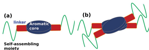
Fig. 1 (a) Schematic representation of key moieties of a monomer & its (b) dimer, exhibiting a helical twist.
