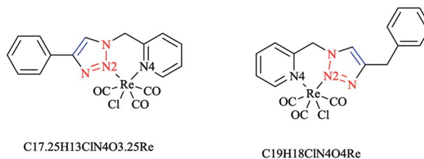
C19H18ClN4O4Re
